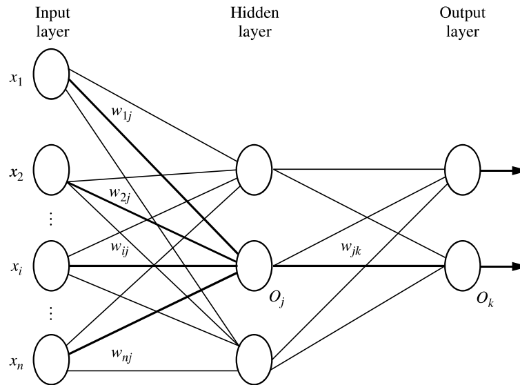
Figure 9.2 Multilayer feed-forward neural network.
